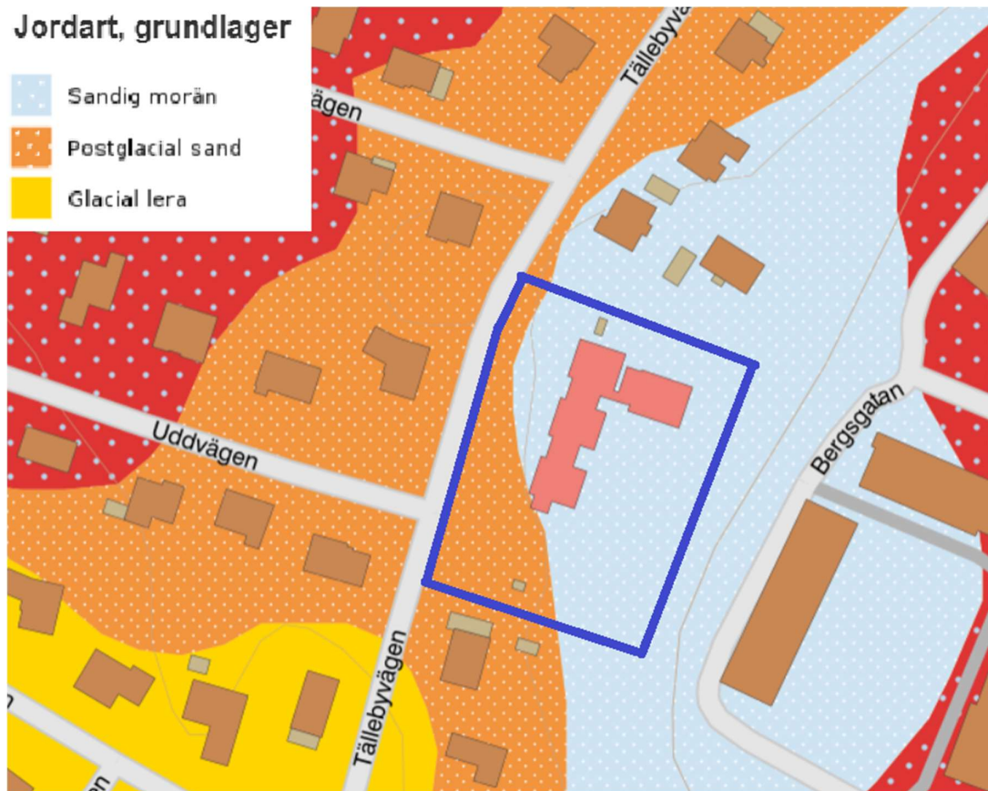
Figur 4. Jordarter (SGU)
